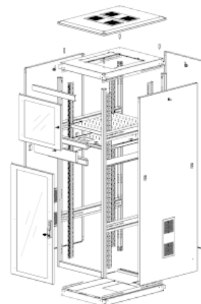
EXPLODED VIEW
